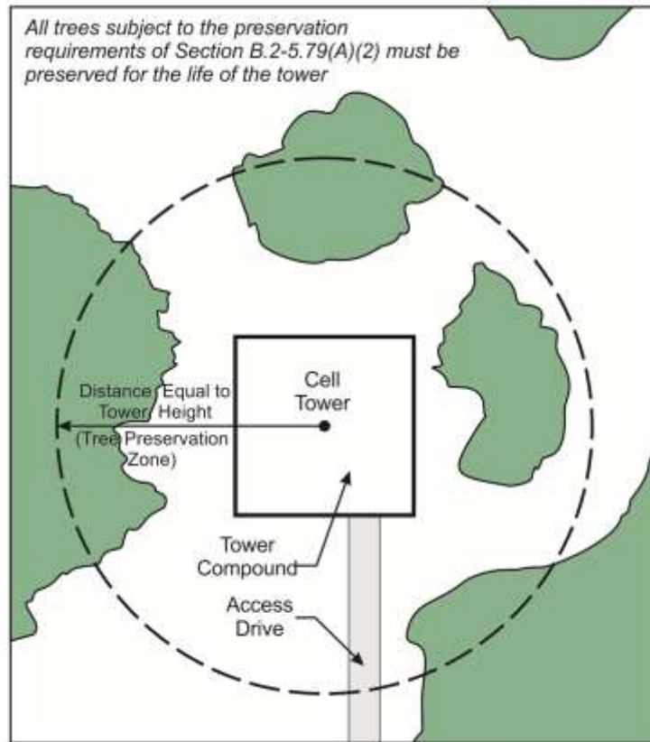
FIGURE 5.2.92: TRANSMISSION TOWER TREE PRESERVATION ZONE
