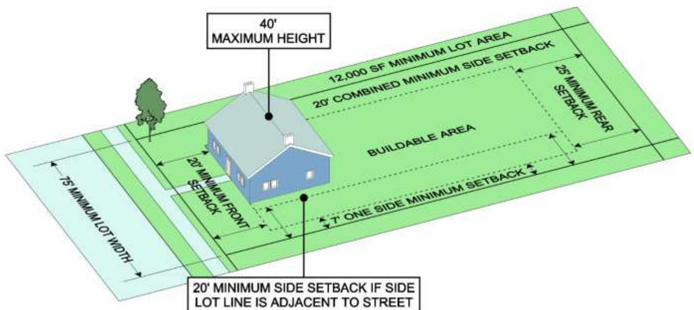
FIGURE 4.5.7.B: GENERAL DIMENSIONAL REQUIREMENTS – RS-12 DISTRICT
