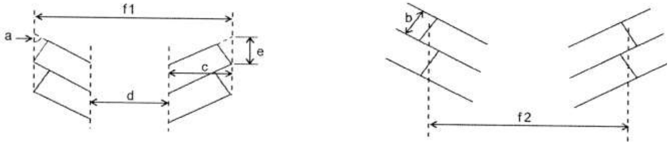
FIGURE 6.1.3.B.1: PARKING DIMENSIONS
