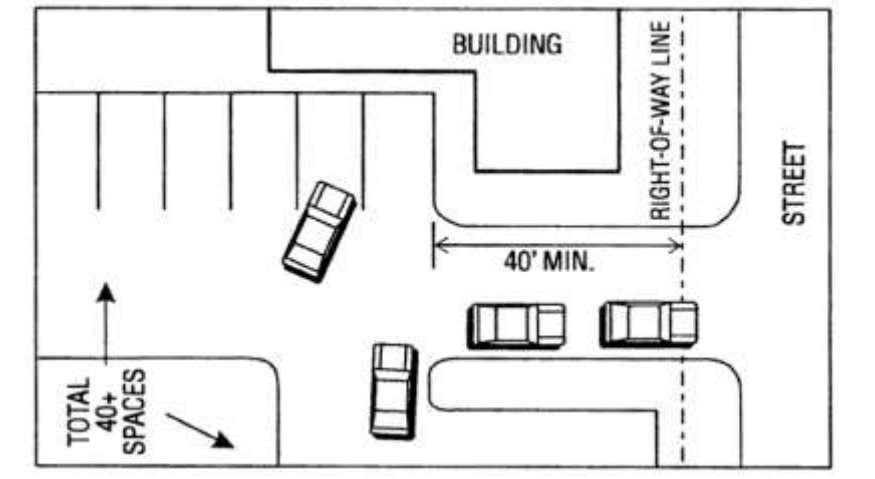
FIGURE 6.1.3.D.4: FRONTAGE ROAD ACCESS
