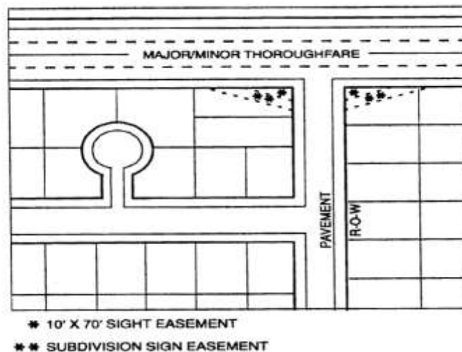
FIGURE 3.2.9.D.4: SIGHT EASEMENTS
