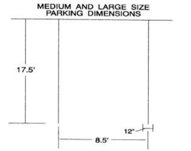
FIGURE 6.1.3.B.2: MEDIUM AND LARGE PARKING SPACES
