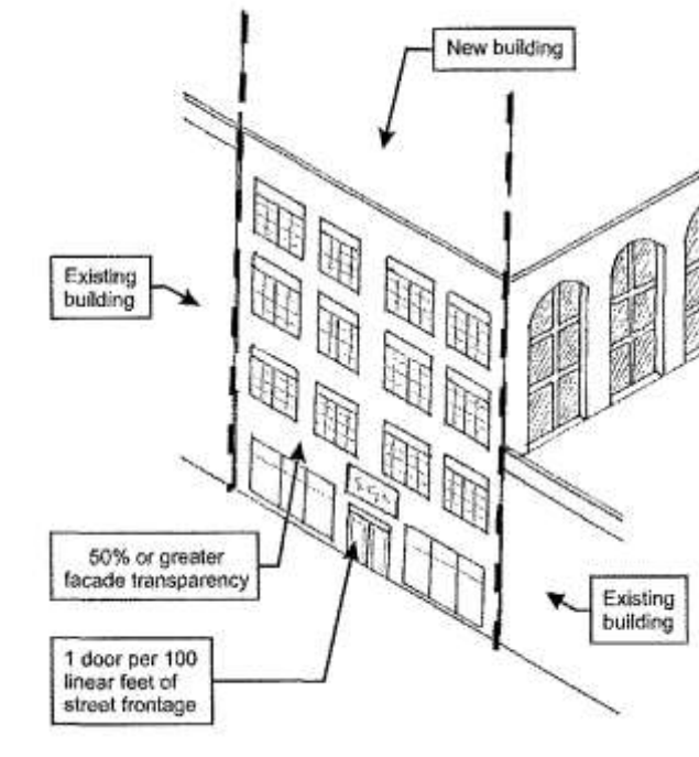
FIGURE 4.9.6.D: STRUCTURES IN THE WO DISTRICT
