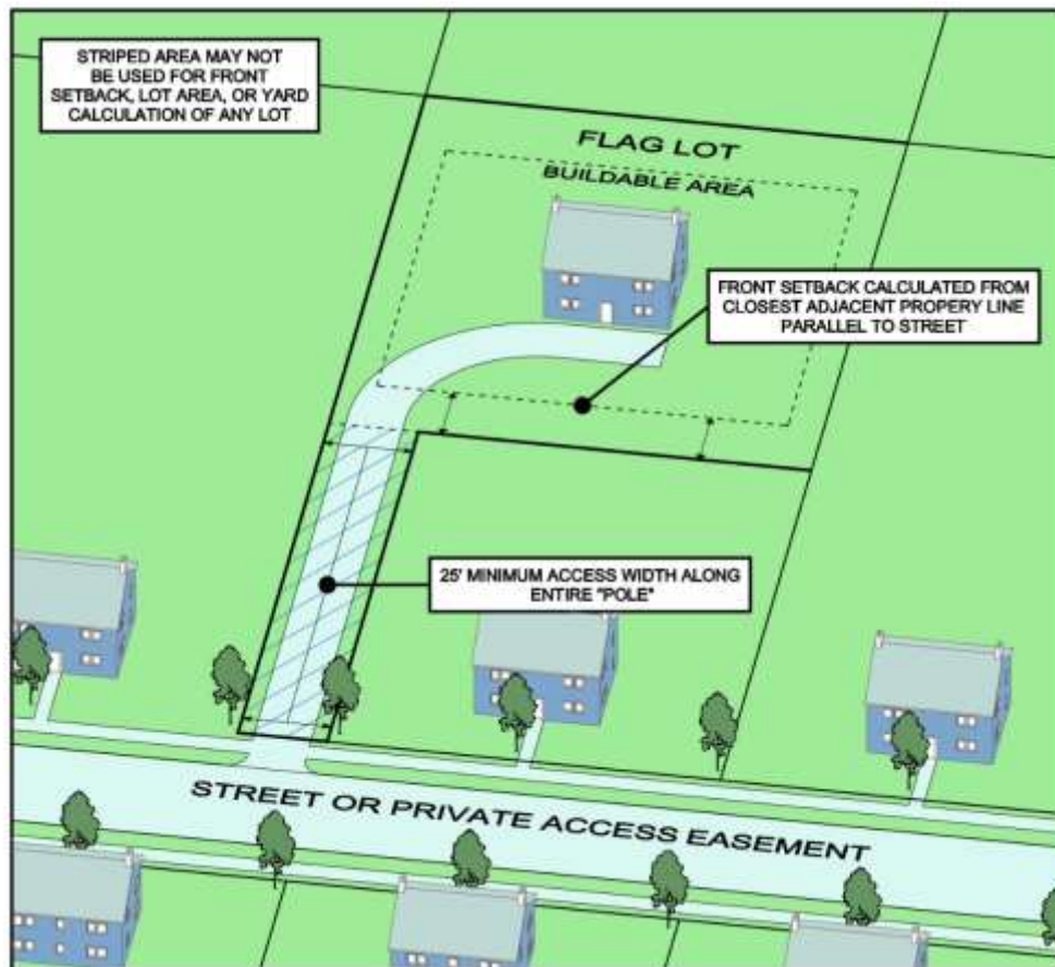
FIGURE 4.1.4.C.14: FLAG LOTS
